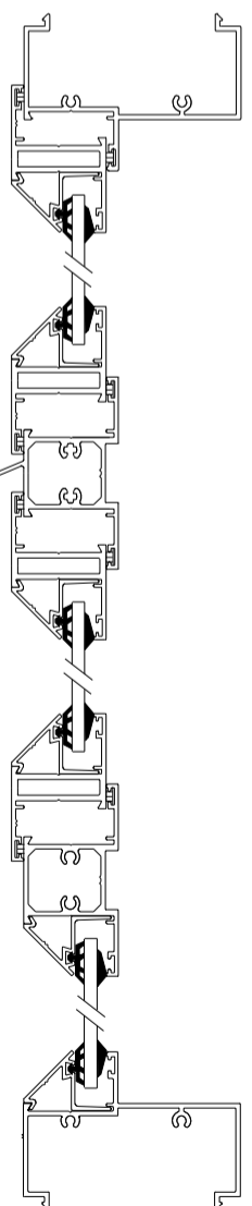
SECTION B-B Section not to scale
