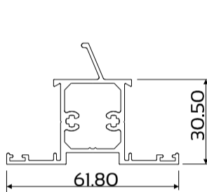
DIE No. W53630 Swift 30.5 Mullion 30mm Weather Bar
