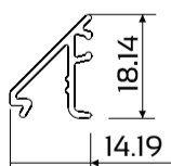
DIE No. W35620 Swift 30.5 Bead Euro 13mm Gap
