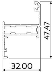
DIE No. W55441 Swift 30.5 Sash Picture Frame
