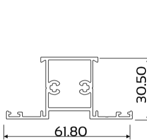
DIE No. W55685A Swift 30.5 Mullion 30mm Standard
