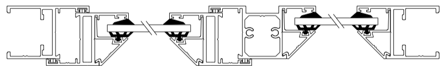
SECTION B-B Section not to scale
