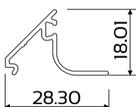
DIE No. W31139A Swift 30.5 Bead Multi 13mm Gap
