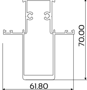
DIE No. W54652A Swift 30.5 Mullion 70mm
