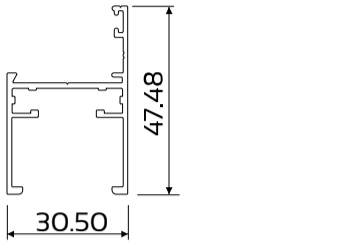
DIE No. W32028A Swift 30.5 Frame 30mm Unequal Leg
