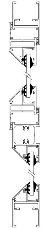
SECTION B-B Section not to scale
