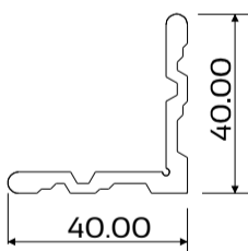
DIE No. W27989 Swift 30.5 Corner Cleat 40mm
