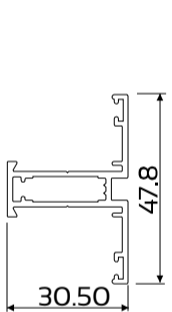
DIE No. W54867 Swift 30.5 30mm Cottage Pane Mullion
